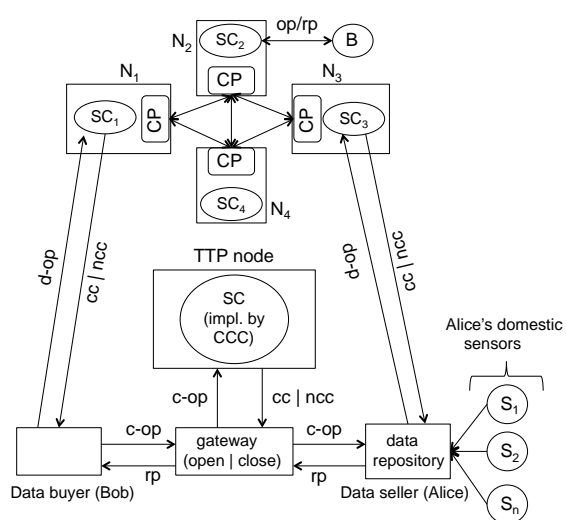
Fig. 5. Hybrid smart contract.
